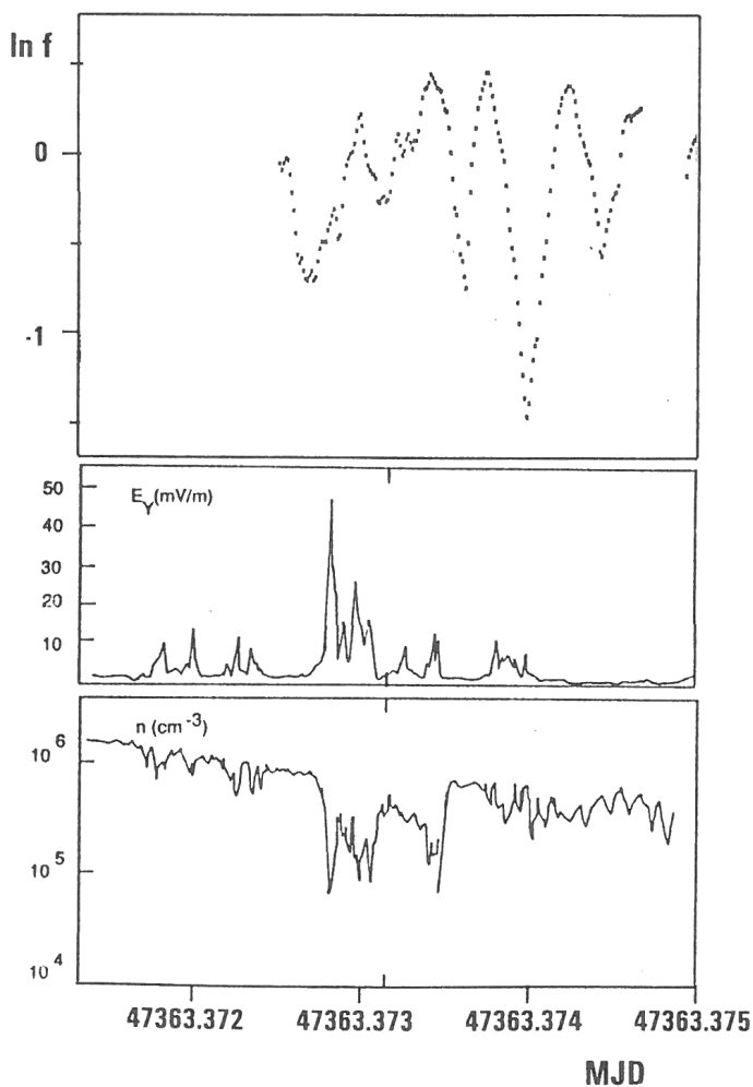
Fig.12. Upper part: variation of neutral density residuals as compared to MSIS'86 model in the time interval corresponding to plasma measurements given in the lower part of this figure. Lower part: variation of the electric field vector and of the plasma density according to Aggson et al. (1992) during an exceptional plasma bubble crossing.
