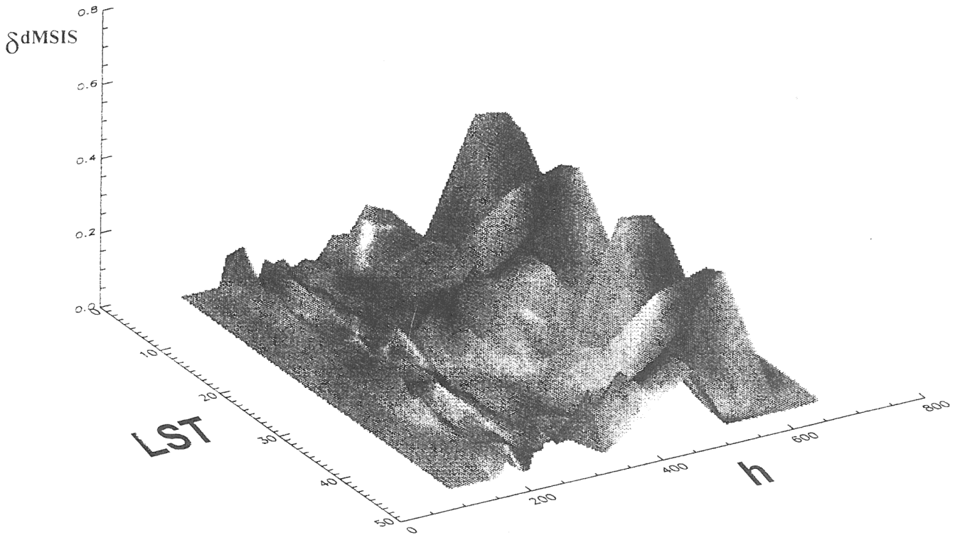
Fig.5. The dependence of the average wave amplitude on LST and height. The average level is fluctuating at low altitudes (San Marco V data).
