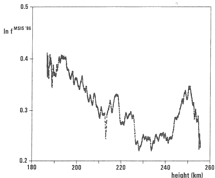
Fig.1. Wave-like fluctuations of different frequencies in the MSIS'86 residuals according to San Marco V data.
