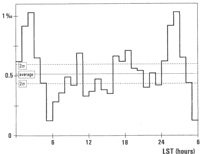
Fig.9. Histogram of sudden density decreases according to LST, normalised as fraction of the total number of observations in every hour interval.
