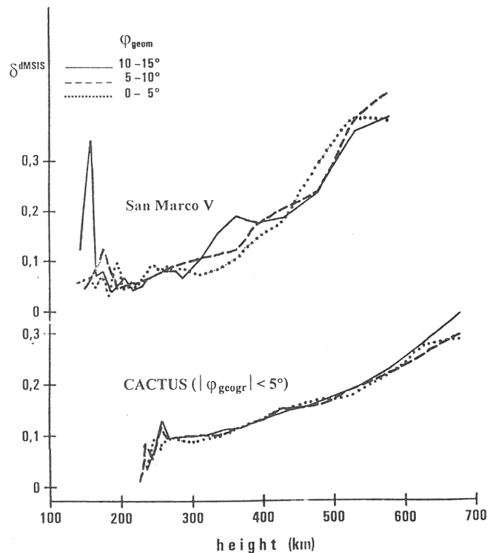
Fig.4. Height dependence of the average wave amplitude for CACTUS and for San Marco V data separated according to geomagnetic latitude. The peak under 200 km (San Marco V) is shifted towards lower altitudes at higher latitudes.
