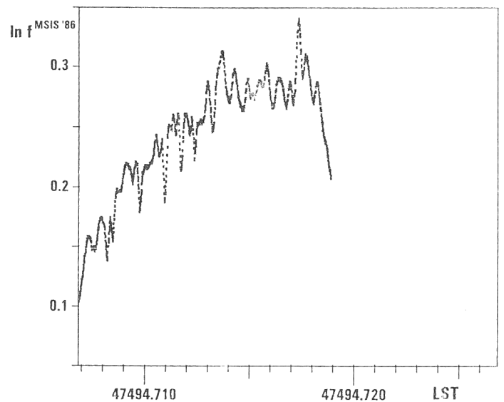
Fig.7. A series of sudden density decreases on a density residual curve.
