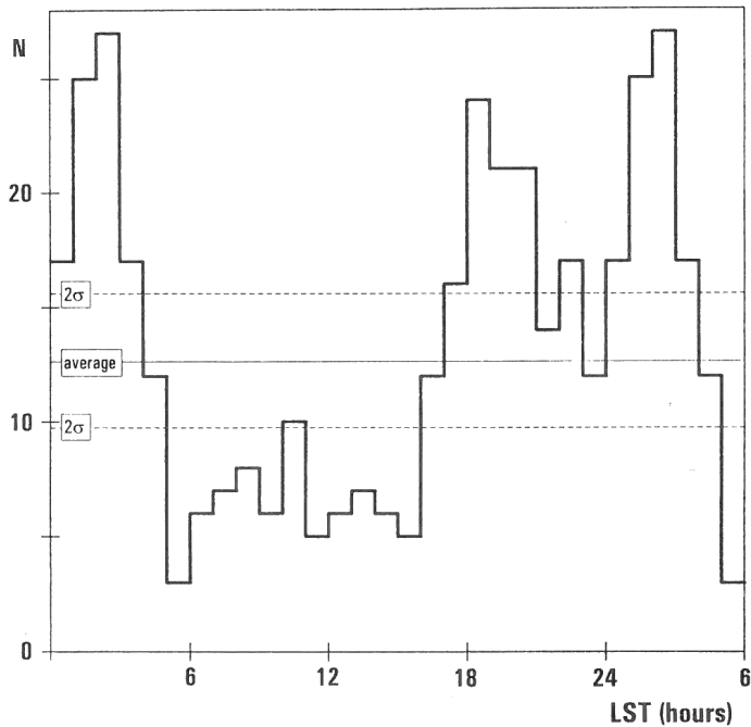
Fig.8. Histogram of sudden density decreases according to LST.
