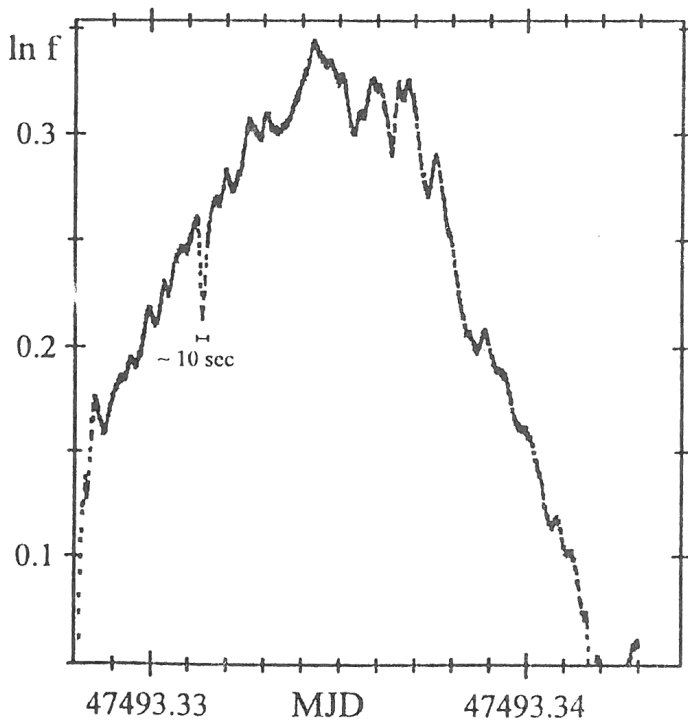
Fig.6. The density residual curve illustrates the occurrence of a typical sudden density decrease phenomenon. MSIS'86 model is used.
