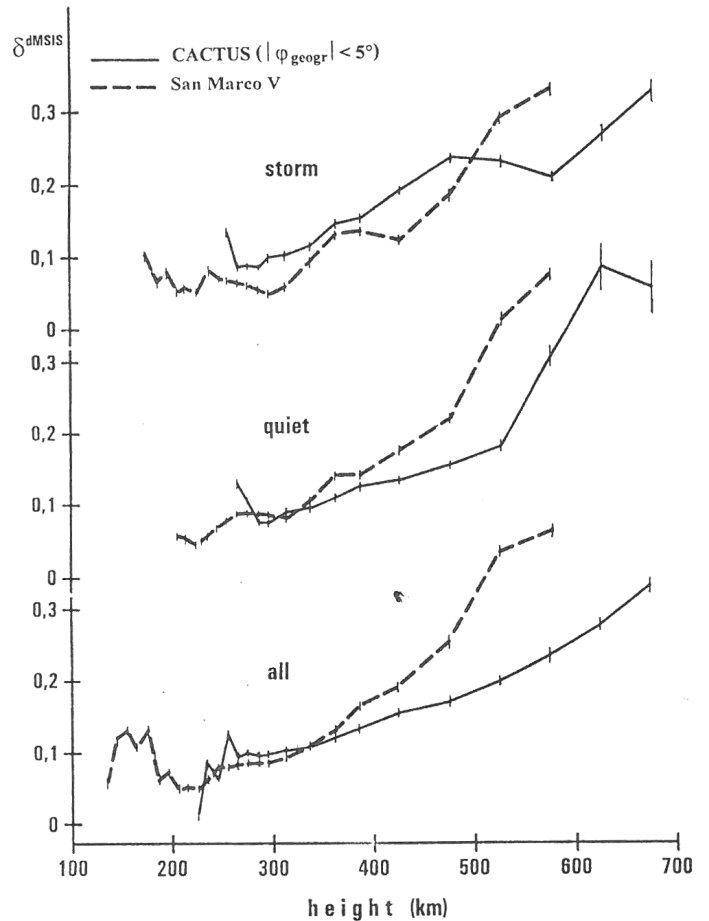
Fig.3. Height dependence of the average wave amplitude for quiet and for disturbed conditions (CACTUS and San Marco V data).
