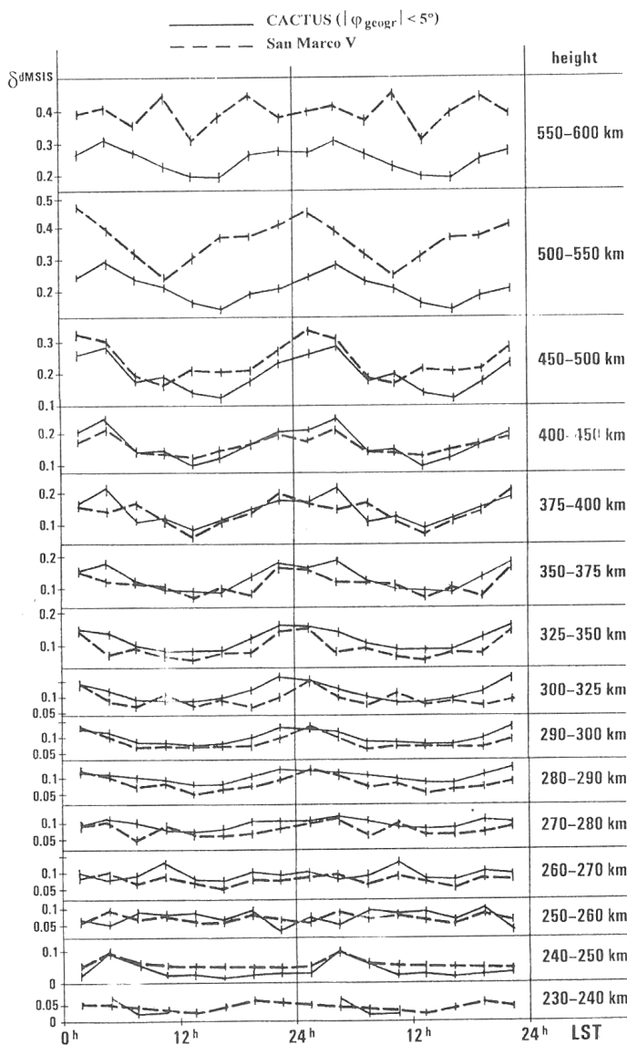
Fig.2. Diurnal variation of the average wave amplitude separated according to height (CACTUS and San Marco V data).
