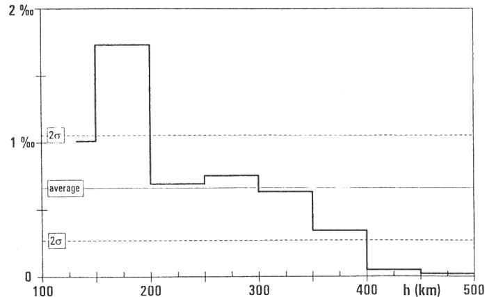
Fig.10. Histogram of sudden density decreases according to height, normalised as fraction of the total number of observations in every height interval.
