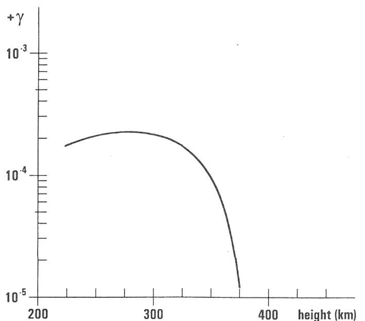
Fig.11. Variation of the growth rate \gamma of the gravitational Rayleigh-Taylor instability with height. The growth rate \gamma is indicated on the vertical axis by a logarithmic scale.
